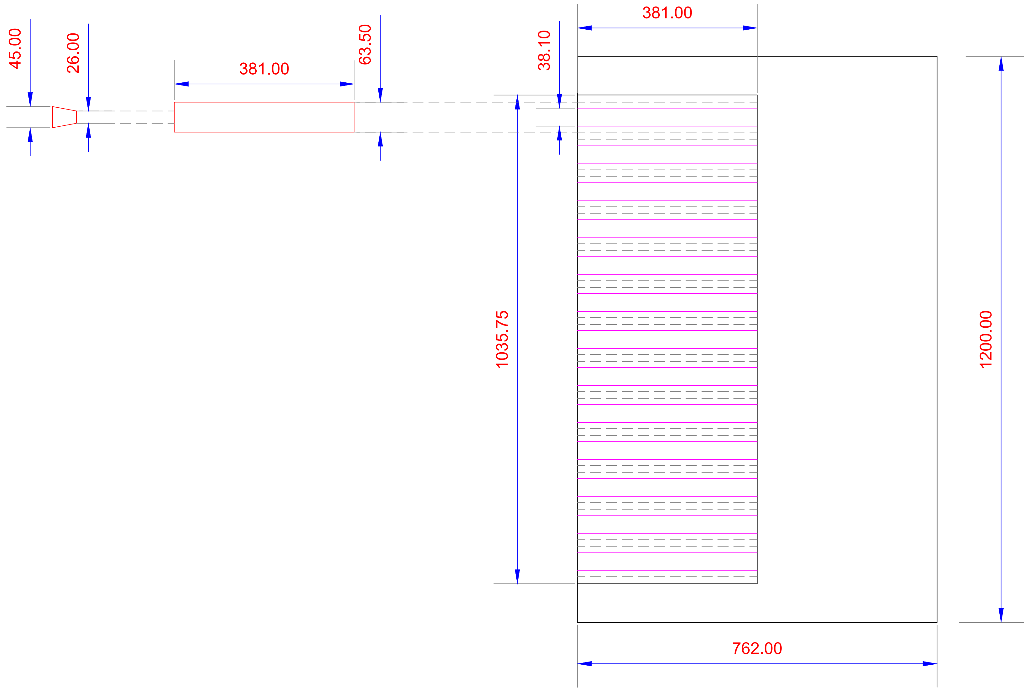
FRONT VIEW
