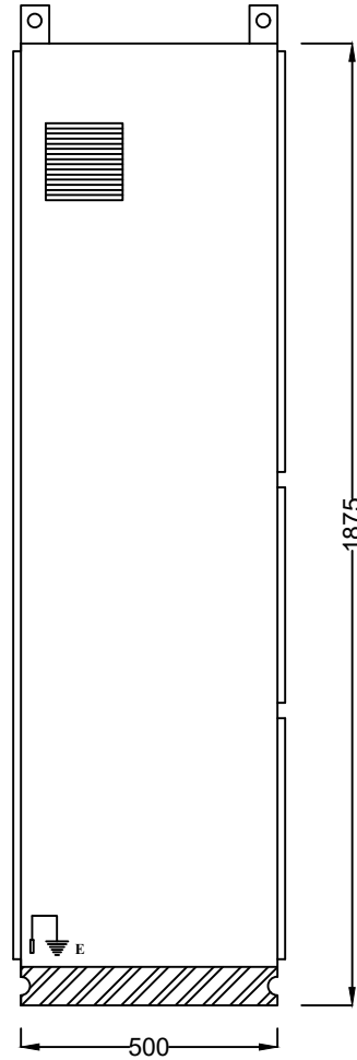
SIDE VIEW
