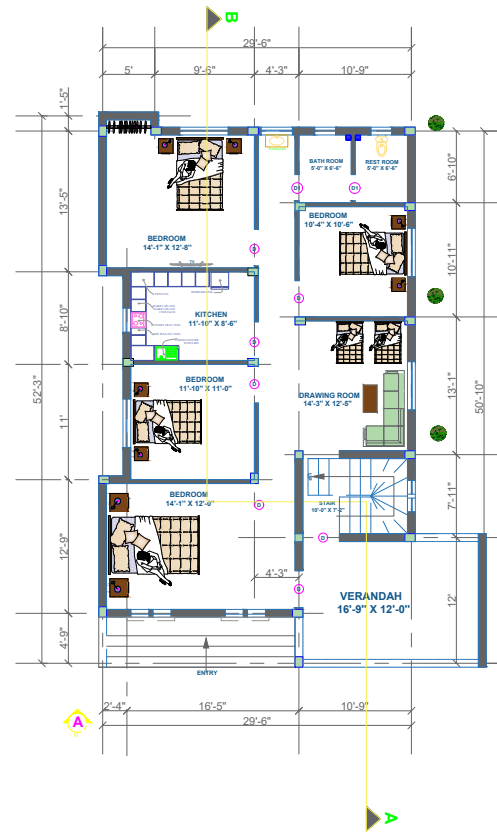
A-GROUND FLOOR PLAN
