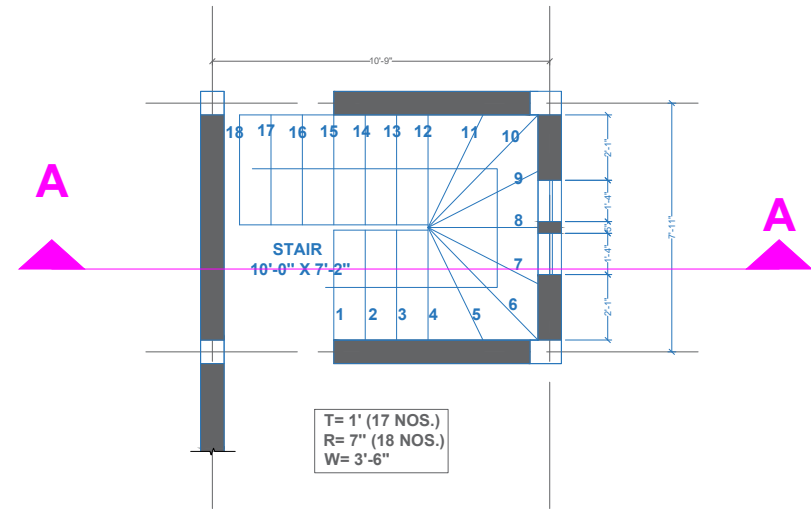
PLAN AT GROUND FLOOR LEVEL
