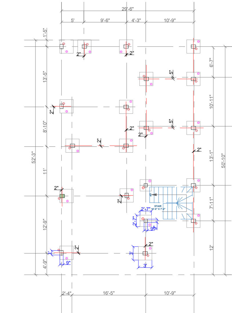
FOOTING/COLUMN LAYOUT PLAN
