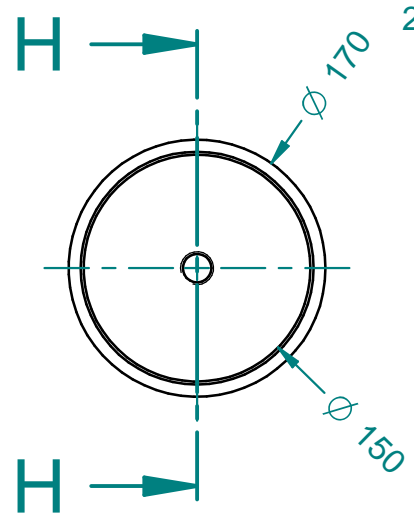
SECTION H-H
