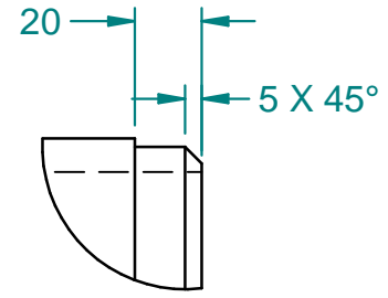
DETAIL F
