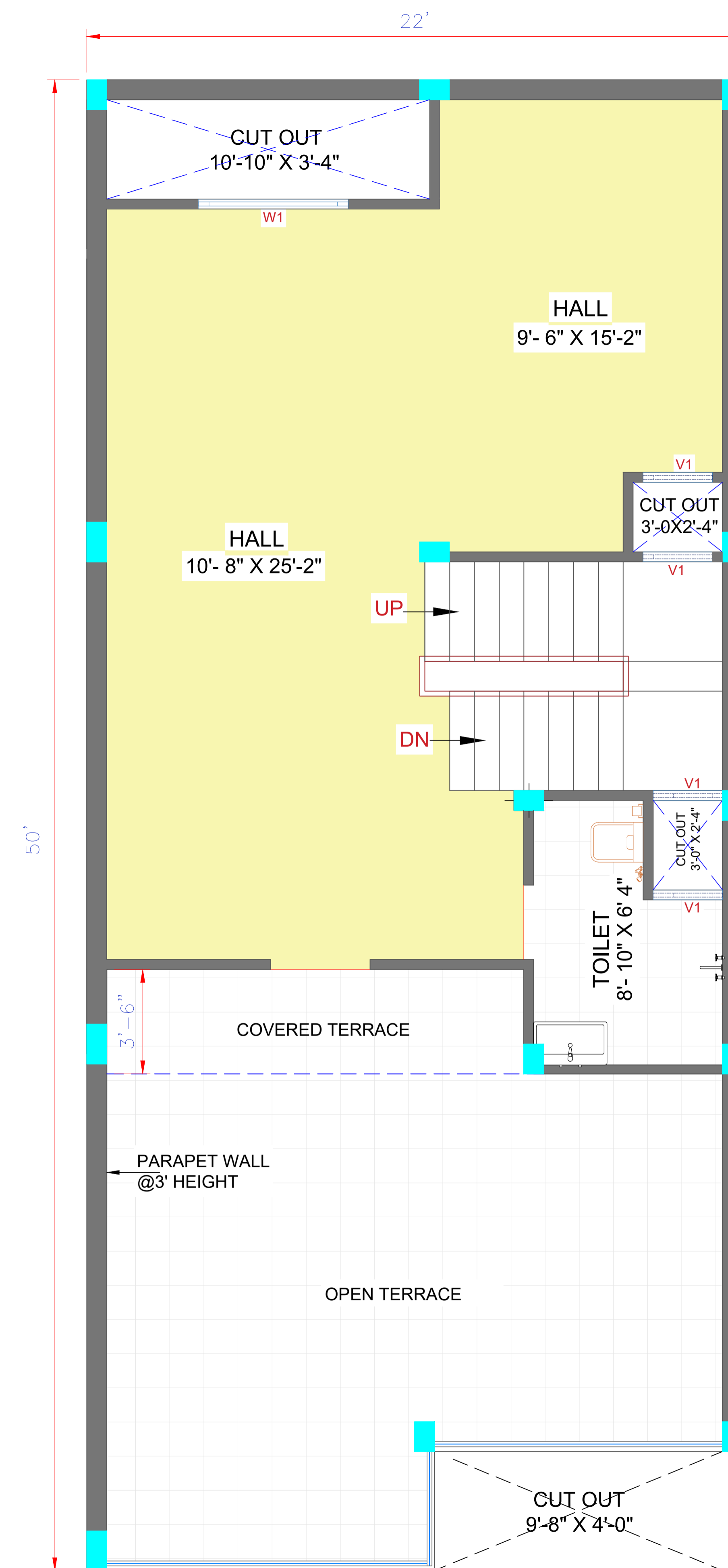
TERRACE PLAN
